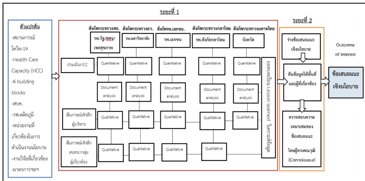
Figure 1 Research framework
